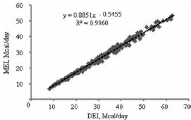
Figure 6. Relationship between digestible energy intake (DEI) and metabolizable energy intake (MEI) expressed as Mcal/day.
