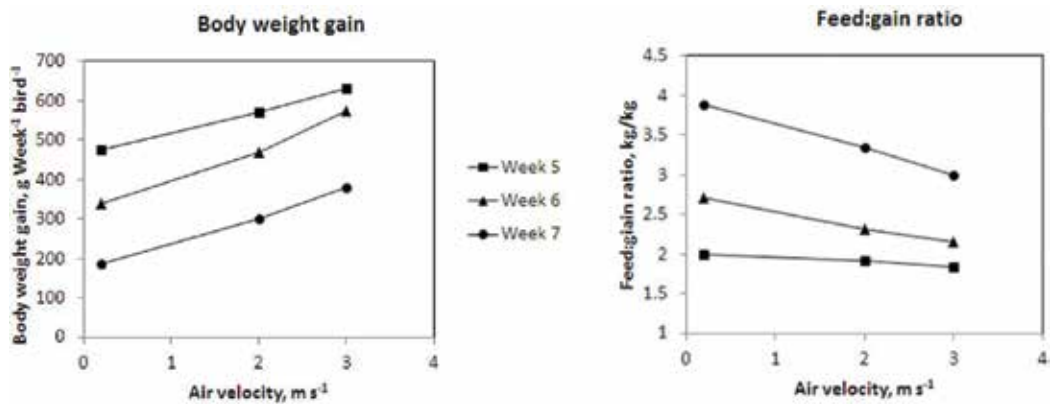
Figure 3. Body weight gain and feed conversion ratio during weeks 5–7 for broilers maintained at different air velocities at air temperatures controlled between 25 and 35°C in a 24-h cycle and at a constant dew point of 23°C [17].
