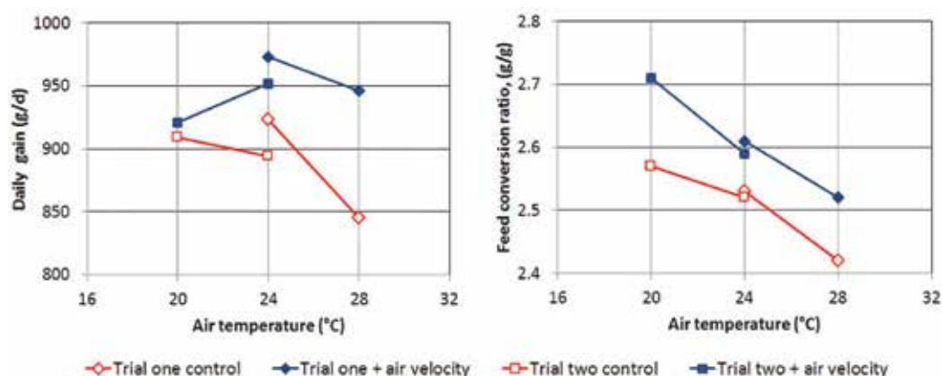
Figure 7. Daily weight gain (left-hand graph) and feed conversion ratio (right-hand graph) for finishing pigs maintained at different air temperatures with and without a ceiling fan to increase the air velocity from 0.56 to 1.3 \text{ ms}^{-1} during the growth period (results reported by Massabie and Granier [22]).
