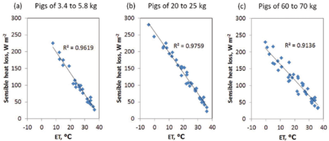
Figure 6. Sensible heat loss for pigs at different ETs calculated by Eq. (7) assuming c = 1 , d = 42^{\circ}\text{C} , 50% RH, and a square-root relationship with measurement. Data originate from mount and Ingram [20] and include exposure to different ambient temperatures (15, 20, 25, 30, and 35^{\circ}\text{C} ) at different air speeds (close to 0.08, 0.35, 0.60, and 1.00 m/s). The three graphs represent different weight ranges.
