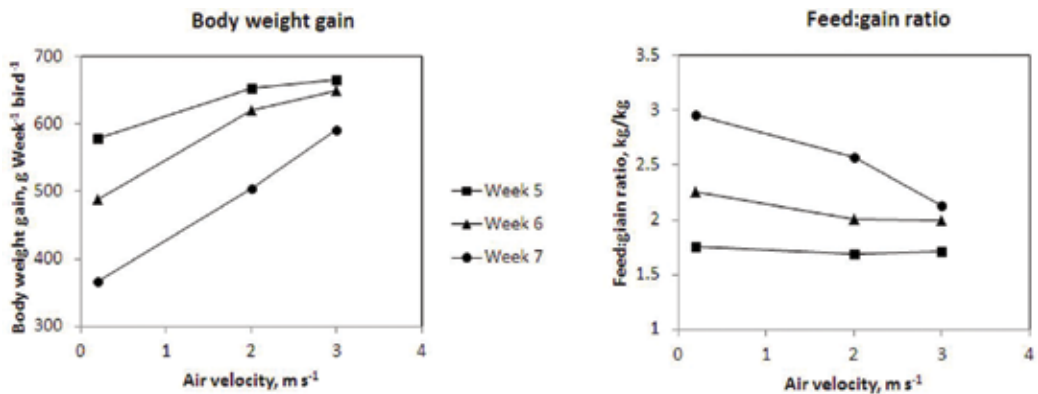
Figure 2. Body weight gain and feed conversion ratio during weeks 5–7 for broilers maintained at different air velocities at air temperatures controlled between 25 and 30°C in a 24-h sine curve and at a constant dew point of 23°C (based on the data by Simmons et al. [11]).
