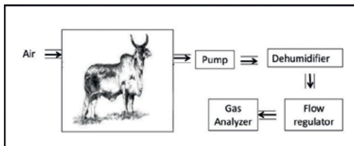
Figure 1. Respirometric chamber's design at LAMACA.
