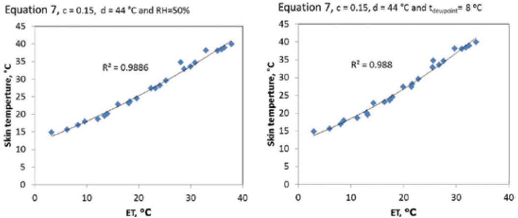
Figure 5. Skin temperature at different ETs calculated by Eq. (7) assuming c = 0.15 , d = 44^\circ\text{C} , and e = 0.5 . Data originate from the study by Uwagawa et al. [13] and include exposure to different ambient temperatures (10, 15, 20, 25, 30, and 35°C) and different air velocities (0, 1, 2, and 4 m/s). The left-hand graph assumes a constant air humidity of 50% RH and the right-hand graph assumes a constant dew-point temperature of 8°C.
