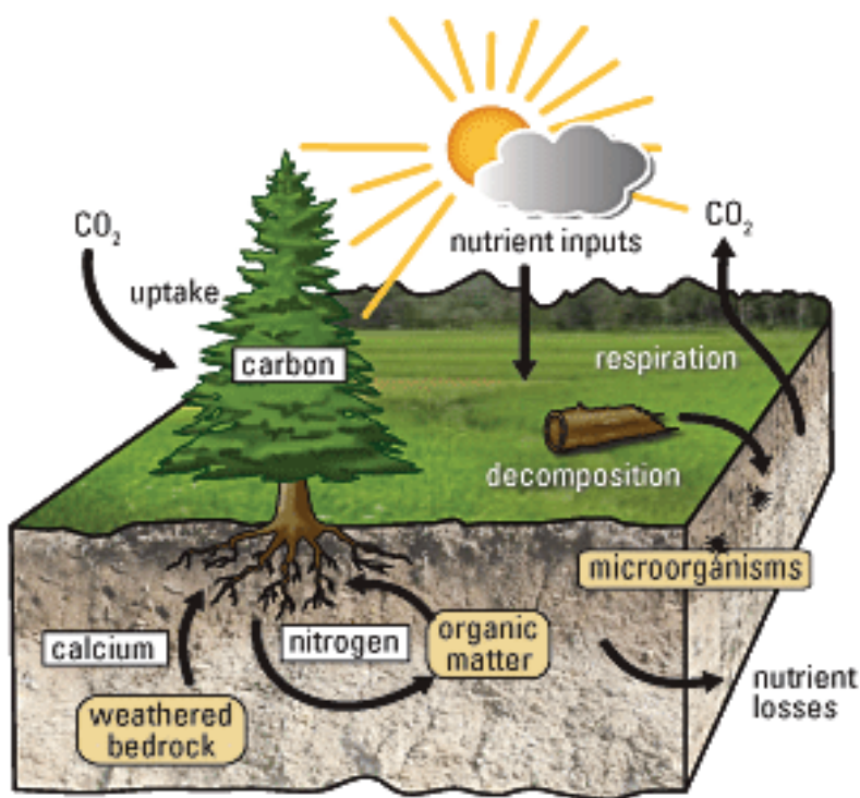
Figure 1. Soil-Plant Nutrient Cycle. This figure illustrates the uptake of nutrients by plants in the forest-soil ecosystem. Source: U.S. Geological Survey.
