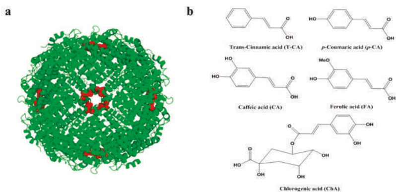
Figure 1. (a) Crystal structure of plant ferritin with views down the four-fold axes (channels) of the protein shell. The tryptophan residue of each subunit is highlighted in red; (b) Chemical structure of cinnamic acid derivatives: Trans -cinnamic acid (T-CA); p -Coumaric acid ( p -CA); Caffeic acid (CA); Ferulic acid (FA); Chlorogenic acid (ChA).
