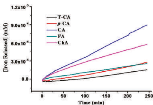
Figure 3. Kinetics of iron release from holo SSF induced by cinnamic acid derivatives. Iron release from SSF in the presence of reductants was followed by measuring the increase in absorbance at 562 nm about 250 min due to the chelation of \text{Fe}^{2+} by ferrozine. Conditions: 0.15 \mu\text{M} SSF, 25 \mu\text{M} cinnamic acids, 50 mM Mops, pH 7.0, 0.15 M NaCl, 500 \mu\text{M} ferrozine, 25 ^{\circ}\text{C} .
